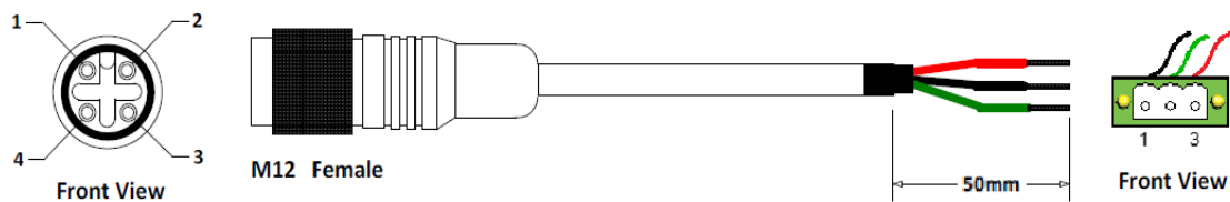
DC Power Input Cable: M12 to 3-pin terminal block
