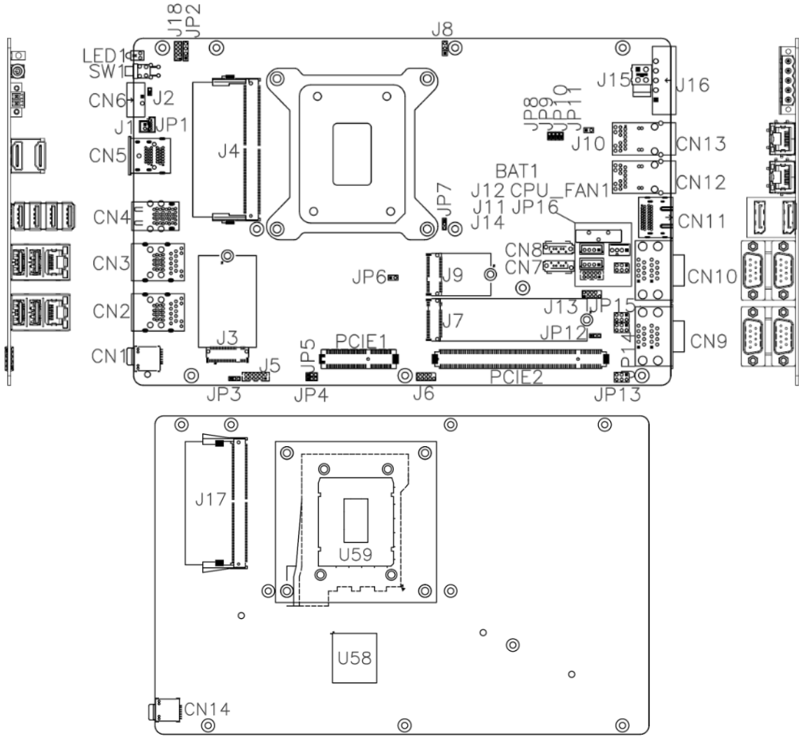
MBE240 Motherboard
