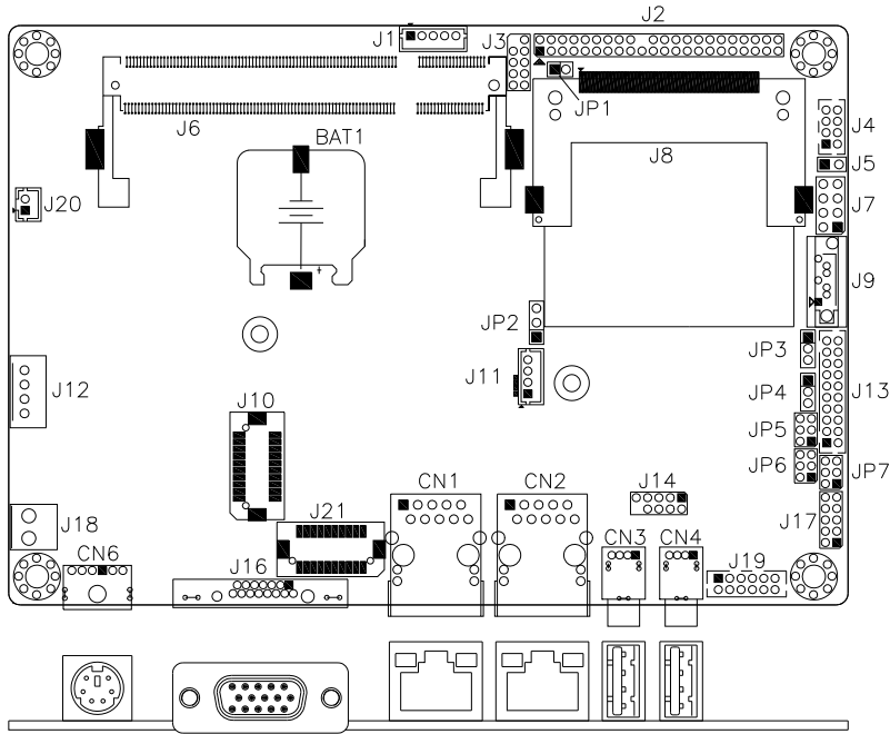
Connector Locations on IB887
