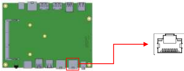
CN10: Gigabit LAN (I217) RJ45 Connector
