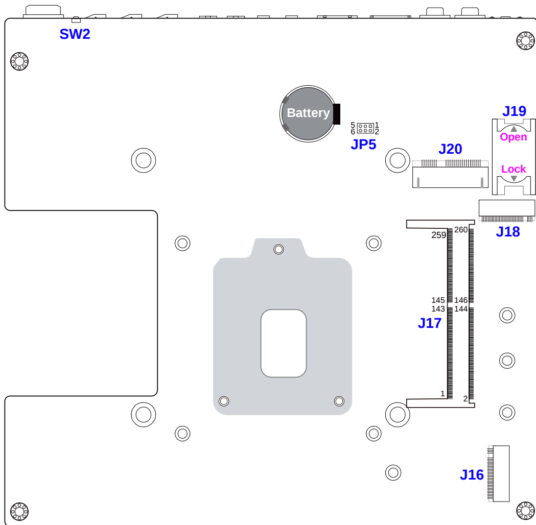
MBD613 - bottom
