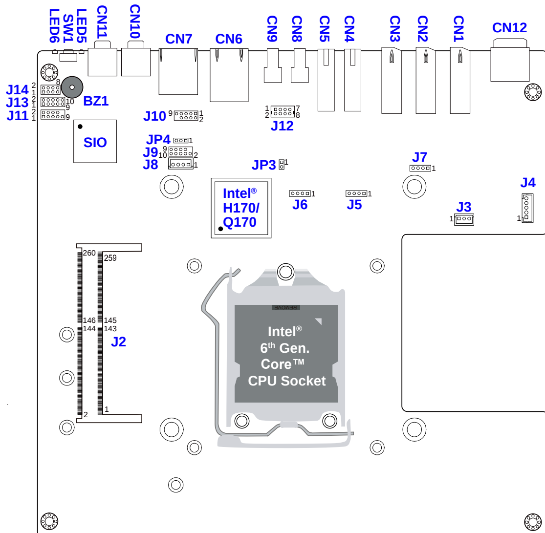
MBD613 - top
