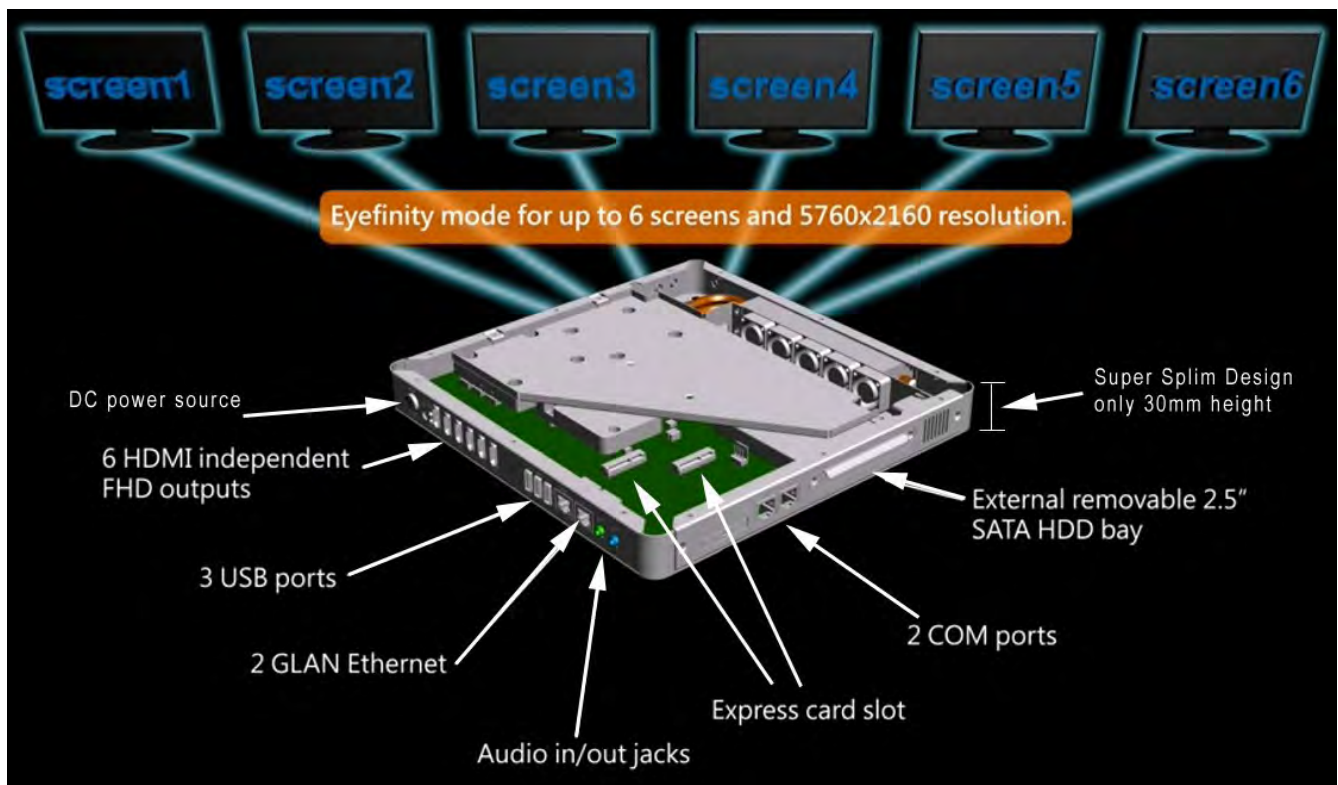
General diagram
