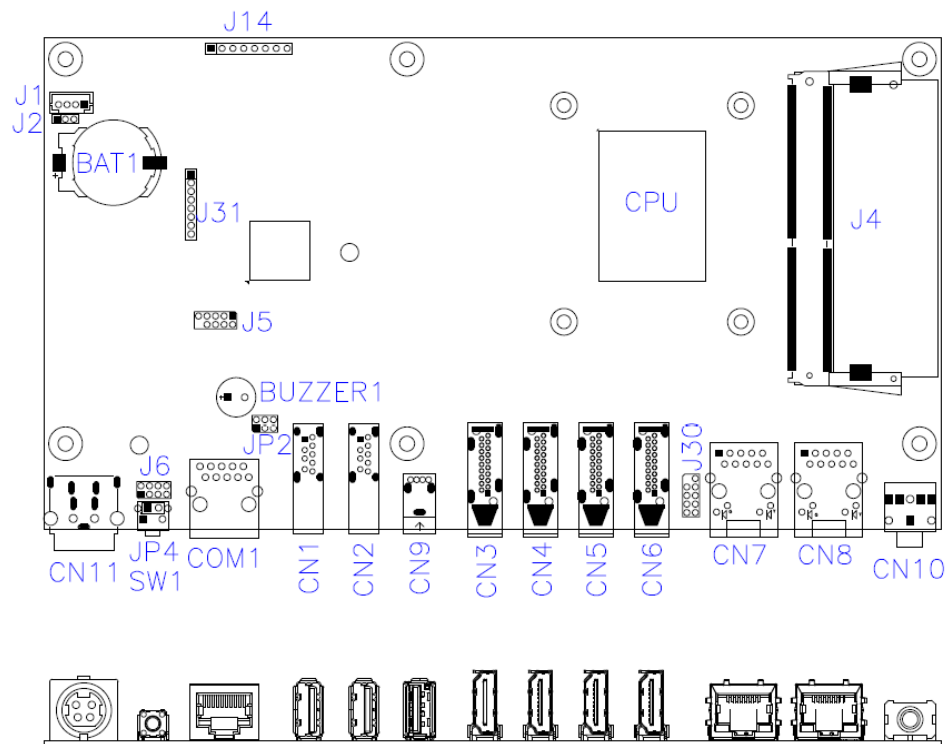
MBD324 – top and I/O
