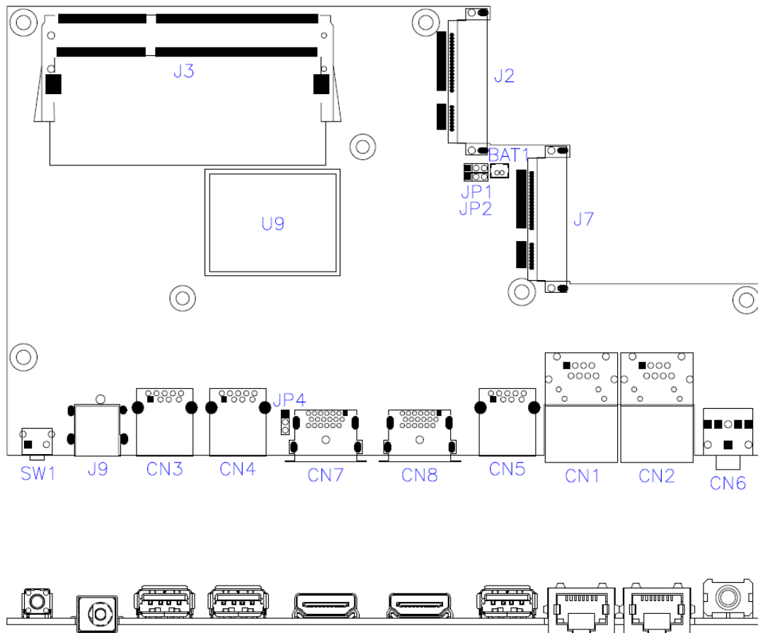
MBD102 – top view
