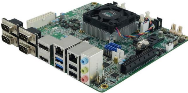
Photo of MI979 (ATX power)
