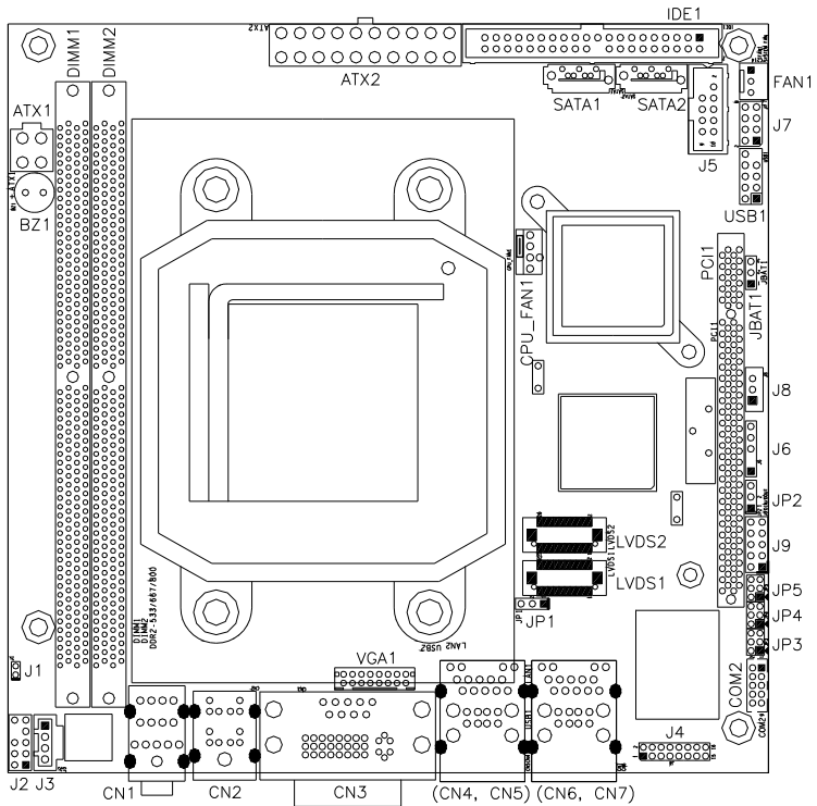
Connector Locations on MI930
