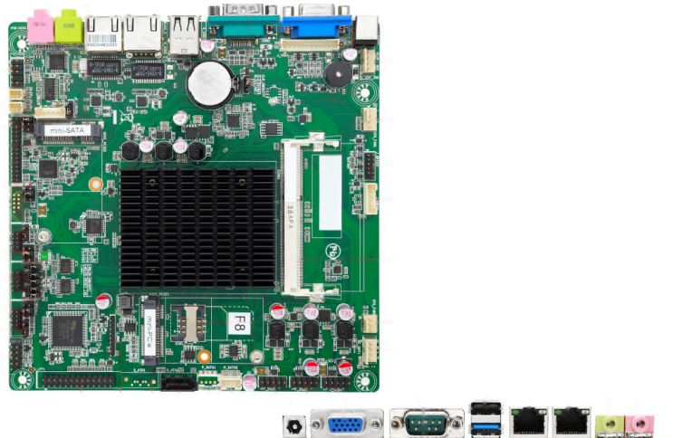
Rear I/O
