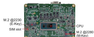
IB961 with heatsink
