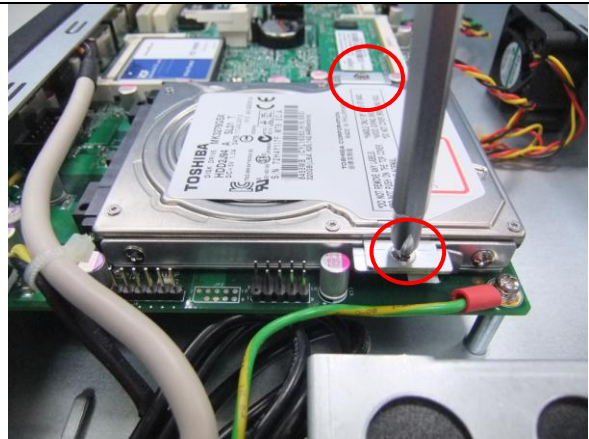
Fig. 8-4 Fix SSD & brackets with two screws
