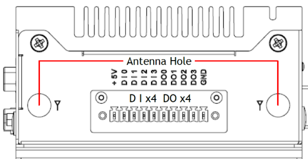
Right Side External I/O
