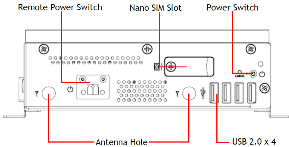
Front External I/O
