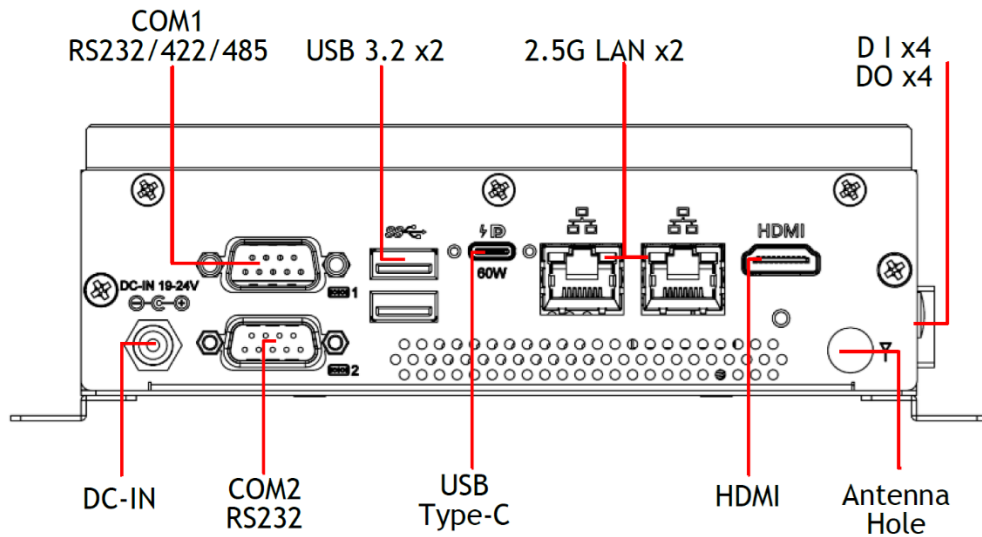
Rear External I/O
