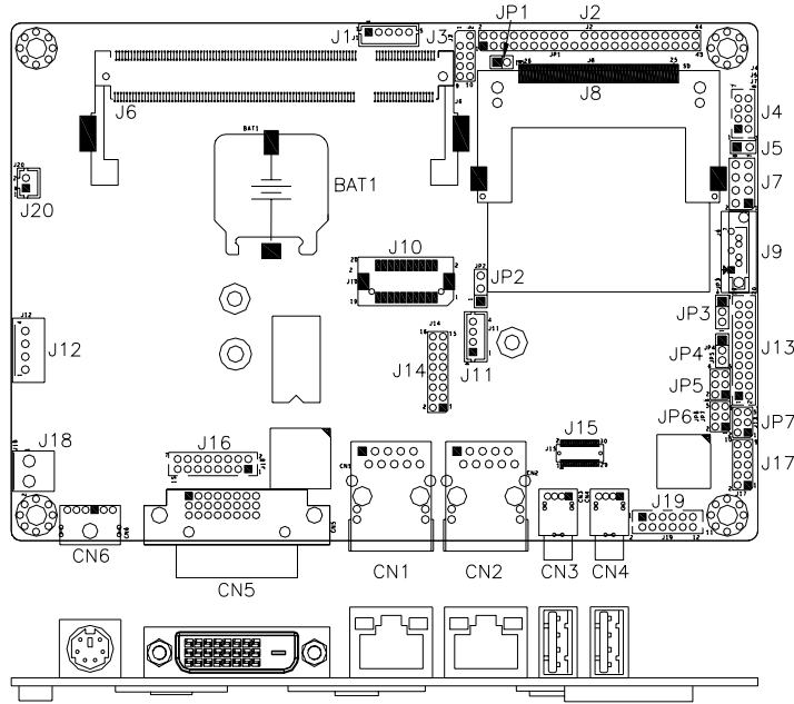
Connector Locations on IB883
